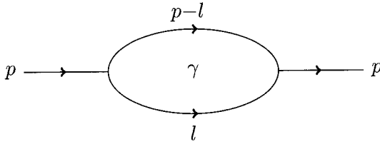
Fig. 17.9 Unsubtracted one-loop propagator graph in \phi_6^3 theory.
