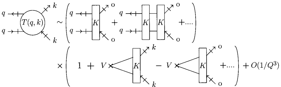
Fig. 18.18 Factorized structure of \mathcal{T}(q, k) at large Q .
