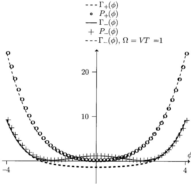
Fig. 14.2 The infinite volume effective potential \Gamma_{\pm}(\phi) for theories defined by action P_{\pm}(\phi) (same parameters as in Fig. 14.1). The effective potential \Gamma_{-}(\phi) at finite volume, \Omega = 1 , for the symmetry-broken case is also shown.
