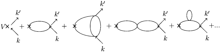
Fig. 18.3 Unsubtracted graphs contributing to \Gamma^{(2,1,1)} up to two loops.
