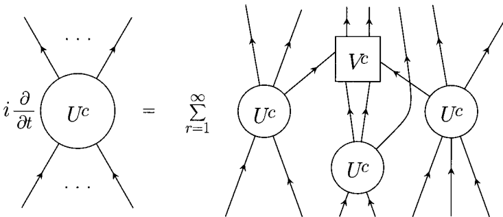
Fig. 6.7 Time development of connected U^c amplitude.
