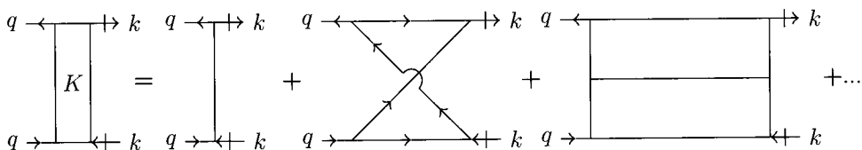
Fig. 18.16 Low-order skeleton graphs contributing to the 2PI kernel K(q, k) .
