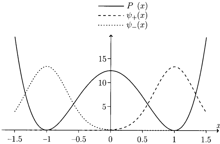
Fig. 14.3 Potential energy function P(x) and approximate ground states \psi_{\pm}(x) for a one-dimensional anharmonic oscillator ( \lambda=300 , m = v = 1 ).
