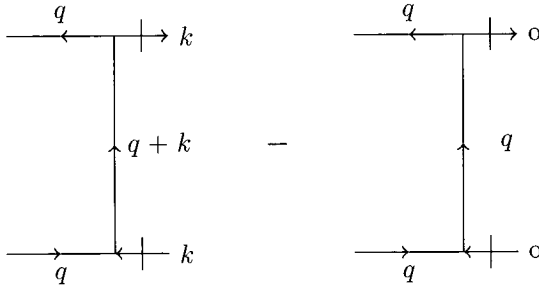
Fig. 18.12 Over-subtraction of the bilocal operator \int d^6\xi e^{iq\cdot\xi} N_4(\phi(\xi/2)\phi(-\xi/2)) .
