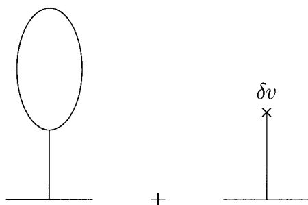
Fig. 17.11 Tadpole graph appearing in \phi_6^3 -theory, and its accompanying counterterm.
