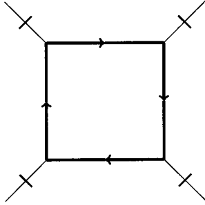
Fig. 17.10 Fermion loop contribution to \bar{\pi} - \bar{\pi} scattering amplitude in Yukawa isospin theory (thick lines are Dirac propagators, thin lines are (amputated) scalar propagators).
