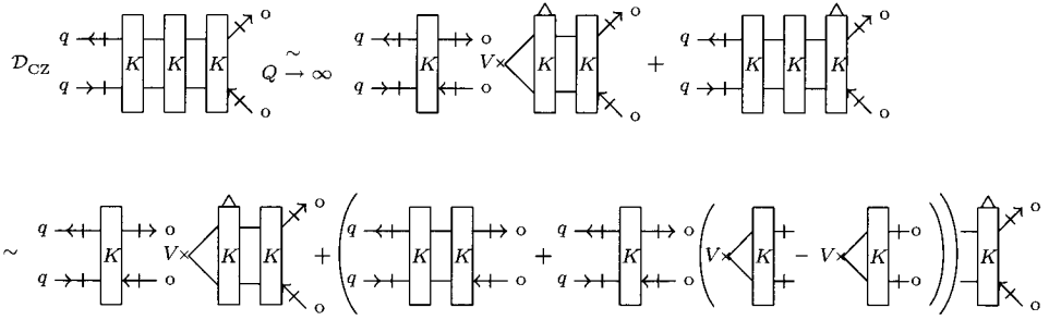
Fig. 18.20 Factorized structure of the three-kernel contribution to \mathcal{D}_{CZ}T(q, 0) at large Q .
