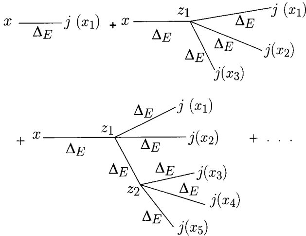
Fig. 10.7 Formal expansion of the classical field \phi_d(x) in powers of j .
