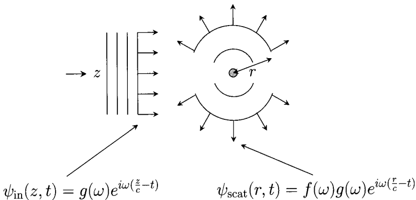
Fig. 6.10 Scattering from a localized target.
