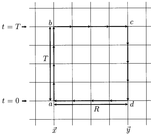
Fig. 19.6 Path corresponding to the Wilson loop observable W(R, T) .
