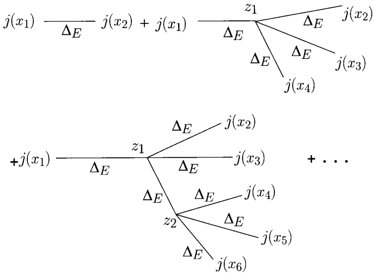
Fig. 10.8 Formal expansion of W_d[j] in powers of j .
