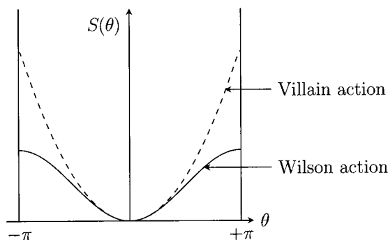
Fig. 19.5 Comparison of Wilson and Villain actions for a U(1) lattice gauge theory.
