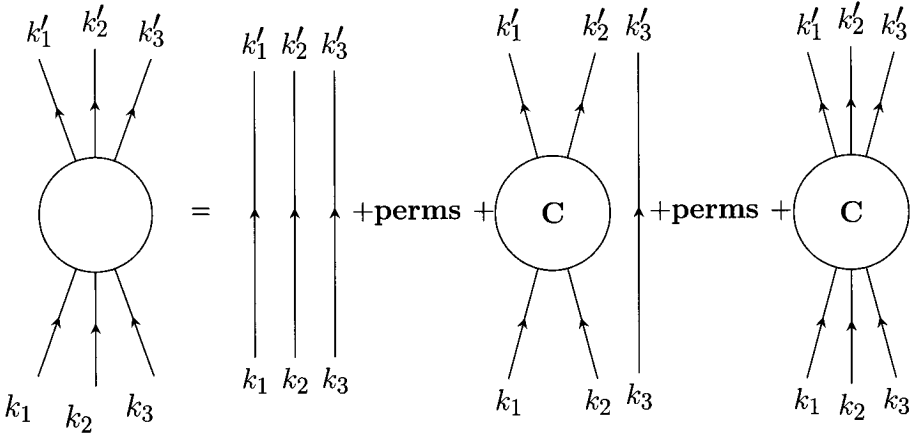
Fig. 6.3 Decomposition of 3-3 S-matrix amplitude into connected parts.
