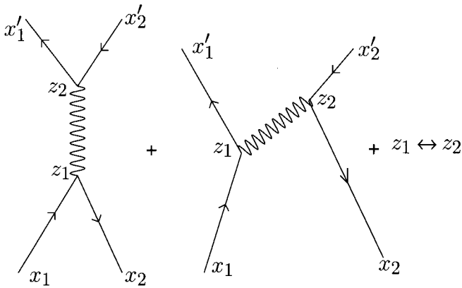
Fig. 10.1 Coordinate space contractions for \psi - \psi^c scattering in second order.
