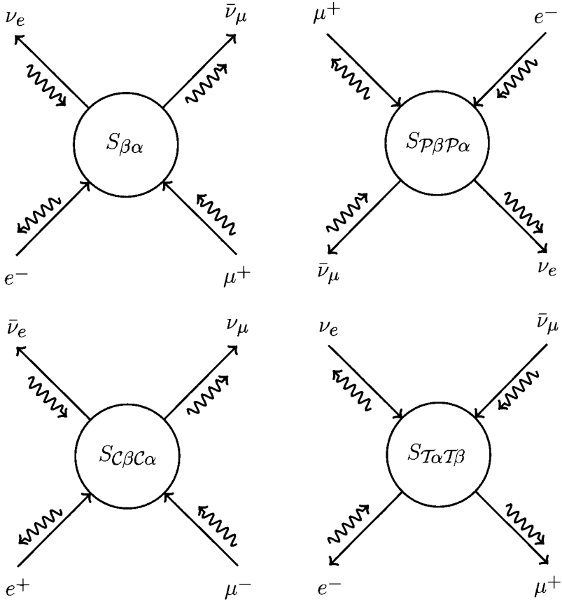
Fig. 13.1 A weak interaction process ( e^- + \mu^+ \rightarrow \nu_e + \bar{\nu}_\mu ) and its \mathcal{P} , \mathcal{C} , and \mathcal{T} transforms. The momentum (straight arrow) and spin (squiggly arrow) vectors are to be taken literally: we have chosen an example with incoming and outgoing particles of definite helicity.
