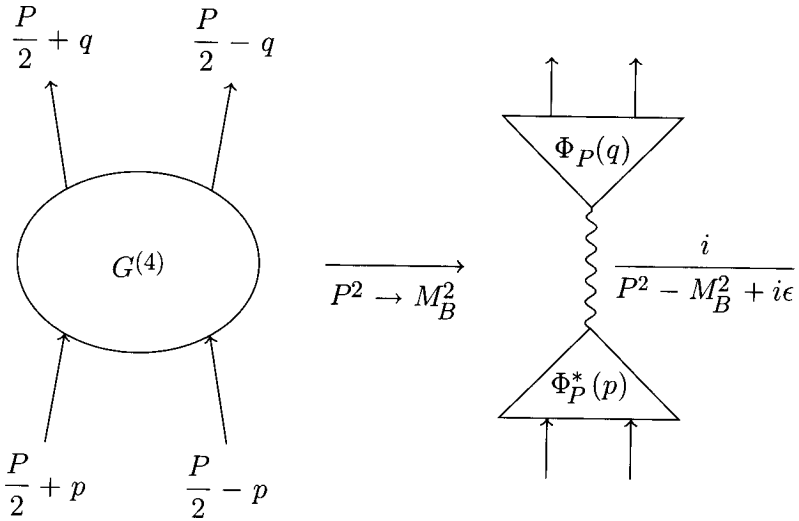
Fig. 11.5 Bound-state pole contribution to the scattering amplitude in a binding channel.
