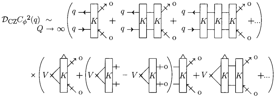
Fig. 18.21 Callan–Symanzik equation for coefficient function \tilde{C}_{\phi^2}(q) , in graphical form.
