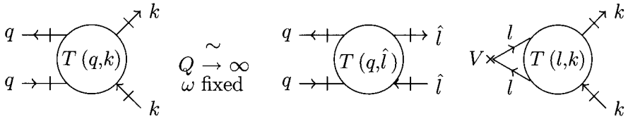
Fig. 18.25 Factorization of \mathcal{T}(q, k) in the Bjorken limit.
