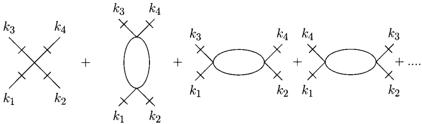
Fig. 17.6 Low-order 1PI contributions (through one loop) to \Gamma^{(4)}(k_1, k_2, k_3, k_4) in \phi^4 theory. The crossbars indicate that external legs are amputated.
