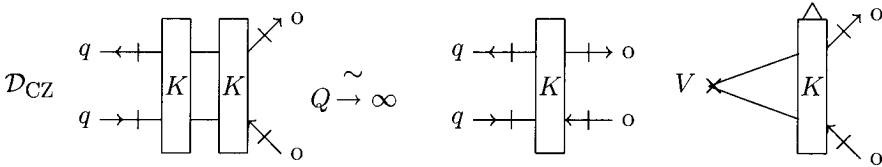
Fig. 18.19 Factorized structure of the two kernel contribution to \mathcal{D}_{CZ}T(q, 0) at large Q .
