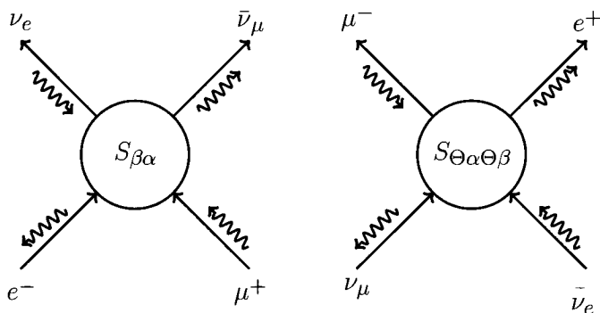
Fig. 13.2 The weak interaction process ( e^- + \mu^+ \rightarrow \nu_e + \bar{\nu}_\mu ) of Fig. 13.1 and its \Theta = \mathcal{TCP} transform. The TCP theorem ensures equality (up to phase) of the amplitudes for the process and its TCP transform in any (weakly) local relativistic quantum field theory describing the interactions responsible for the process.
