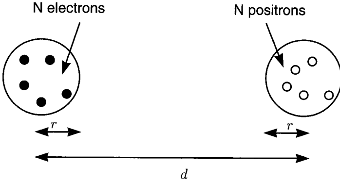
Fig. 11.1 Electron–positron pair assembly leading to energetic instability (for \alpha < 0 ).
