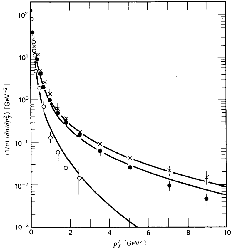
Fig. 11.11 The transverse momentum distribution d\sigma/dp_T^2 of hadrons relative to the thrust axis for different e^-e^+ center-of-mass energies Q : ( \circ ) Q = 12 GeV; ( \bullet ) 27.4 \leq Q \leq 31.6 GeV; ( \times ) 35.0 \leq Q \leq 36.6 GeV. The curves are a QCD calculation. Data are from PETRA.
