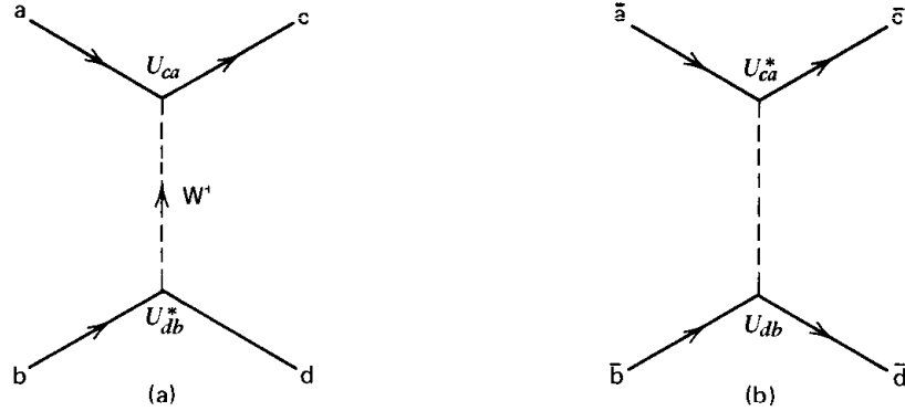
Fig. 12.20 The processes described by (a) the weak amplitude \mathcal{M}(ab \rightarrow cd) and (b) its hermitian conjugate.
