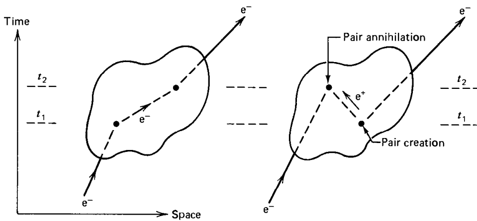
Fig. 3.2 Different time orderings of the double scattering of an electron.
