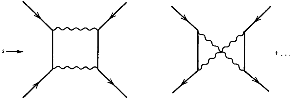
Fig. 6.7 Some higher-order diagrams for e^-e^+ \rightarrow \mu^+\mu^- .
