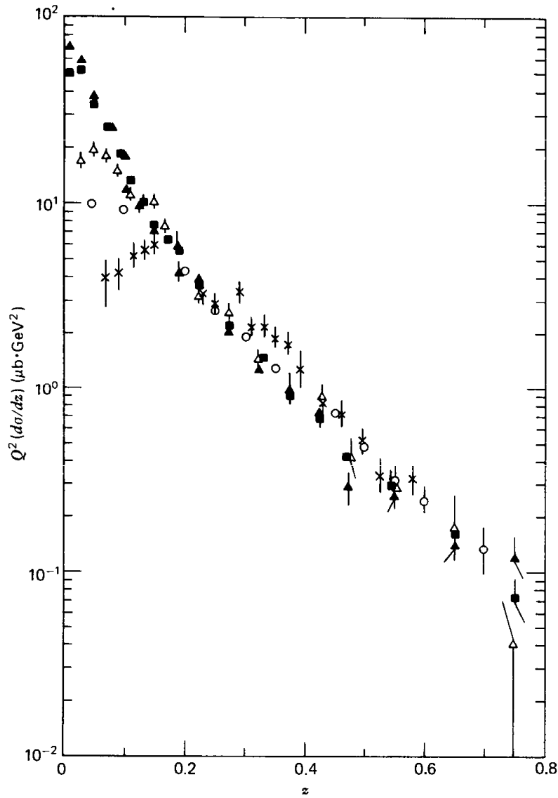
Fig. 11.5 Q^2(d\sigma/dz) \sim 1/\sigma(d\sigma/dz) for e^-e^+ \rightarrow hX as measured as a function z at different center-of-mass energies Q : (×) 5 GeV; (○) 7.4 GeV; (Δ) 12 GeV; (■) 27.4–31.6 GeV; (▲) 35.0–36.6 GeV. Data are from the Stanford Linear Accelerator and PETRA.
